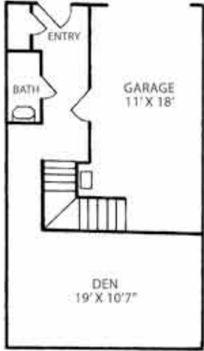
TYPE 2 "L-STAIR" REAR LOAD FOUNDATION PLAN (FRONT LOAD PLAN ALSO AVAILABLE)
